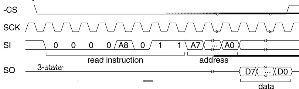
Figure 3. The NM25C04's SPI interface is similar to Microwire's. SCK's falling edges latch inputs at SI, while rising edges clock data out on SO.
